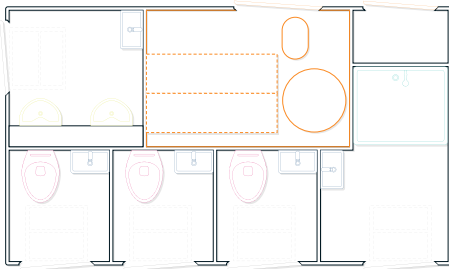
GL4200 TANK 1x SHOWER, 3 SINGLE TOILET CABINS, 1 URINAL CABIN, STORAGE COMPARTMENT
