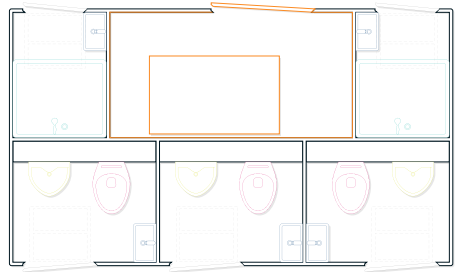
GL4200 TANK 2x SHOWER, 3 SINGLE TOILET CABINS WITH URINAL
