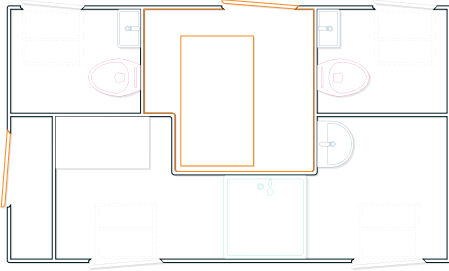
GL4200 TANK 1x MOBILE DECONTAMINATION UNIT, SINGLE TOILET CABINS, URINAL COMPARTMENT
